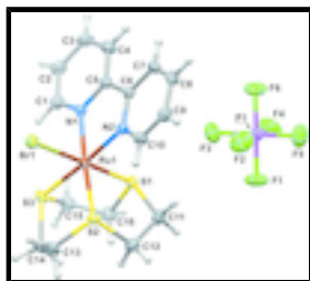
Fig. 1. Asymmetric unit of the title compound, with non-hydrogen atoms represented as displacement ellipsoids drawn at the 70% probability level and hydrogen atoms as small spheres with arbitrary radii. The labelling scheme is provided for all non-hydrogen atoms.
